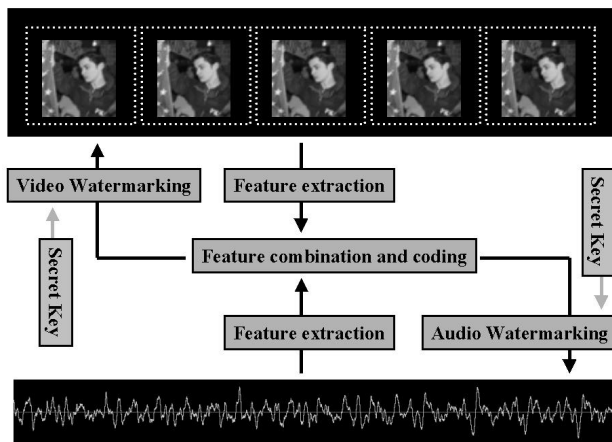
Figure 2: Combined video and audio watermarking based on feature extraction.
